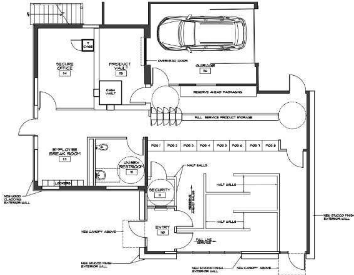
01 FIRST FLOOR PLAN SCALE: 1/8" = 1'-0"
